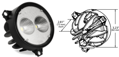
64F11 - Flush Mount
