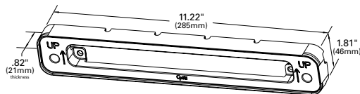
Spacer/Wire Guide
