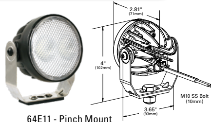
64E11 - Pinch Mount
